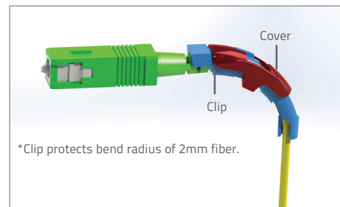
Complete installation of Fiber Marker Clip with special services cover.
