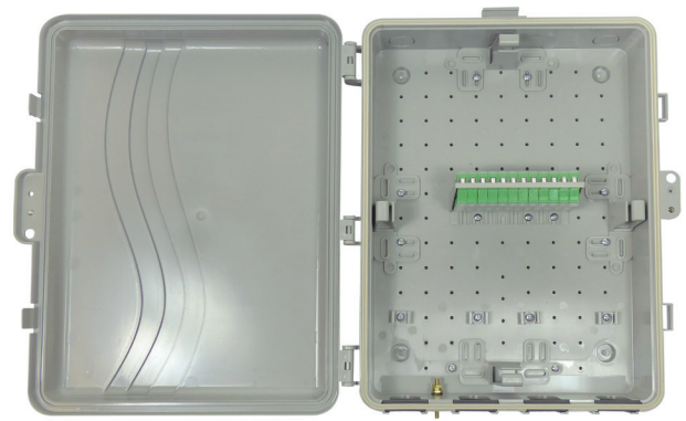
125-1501: 24 SC/APC simplex adapters, gasket, hex bolt, 4 Hurricane Clips, PVC
