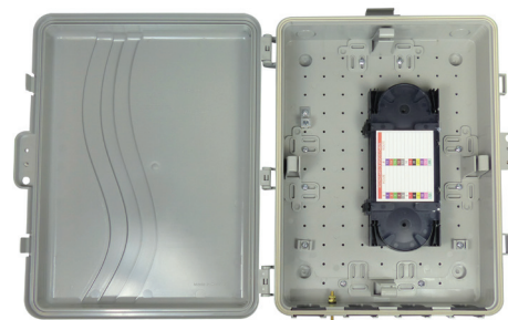
125-1502: 2x12 splice tray, gasket, hex bolt, 4 Hurricane Clips, PVC
